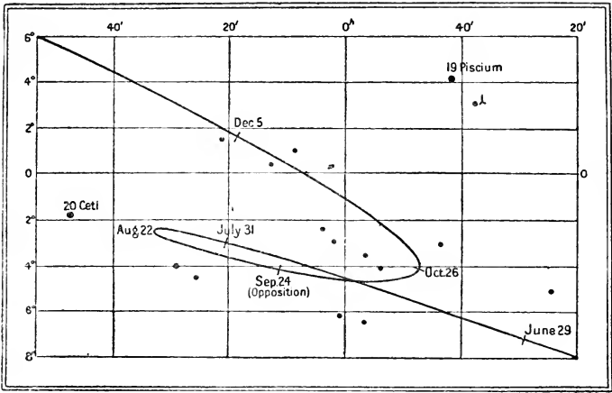
Fig. 28. The Path of Mars among the Stars, 1909.
